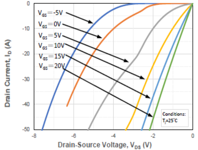
Figure 8. Reverse Output Characteristics at Tj = 25°C
